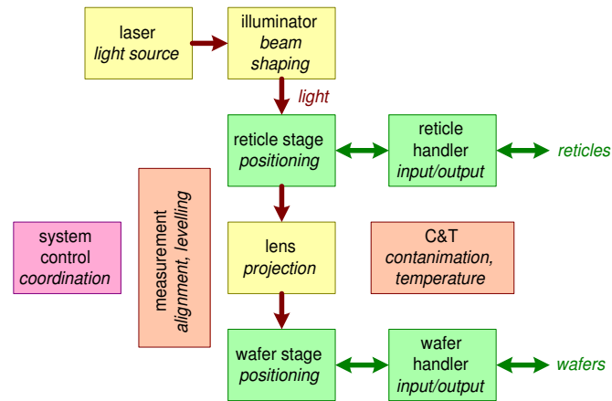
Figure 24: Block Diagram of a Waferstepper
