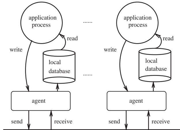
Fig. 1. Splice applications.
