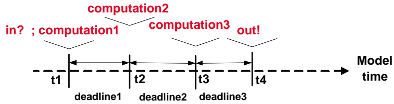
Figure 1.11 Observational equivalent model timed trace
