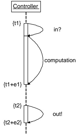
Figure 1.9 Implementation of the controller in physical time
