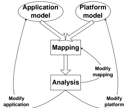
Figure 1.10 Y-chart scheme for real-time systems design
