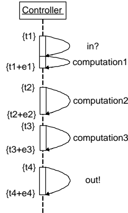
Figure 1.12 Implementation of the equivalent model in physical time
