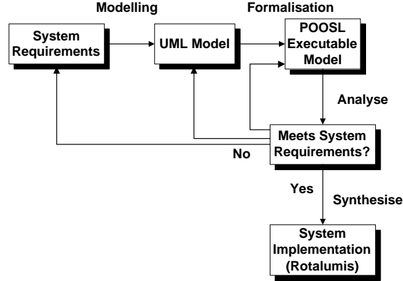
Figure 1.1 SHE method for real-time systems design
