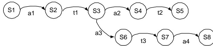
Figure 1.2 Example of a timed labelled transition system
