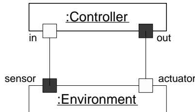
Figure 1.5 The UML model of a simple controller
