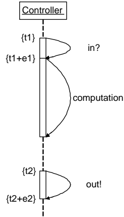
Figure 1.13 A possible execution that still preserves the properties
