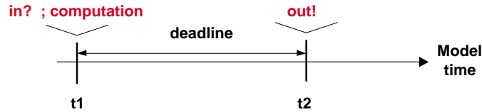
Figure 1.7 A timed trace of the controller
