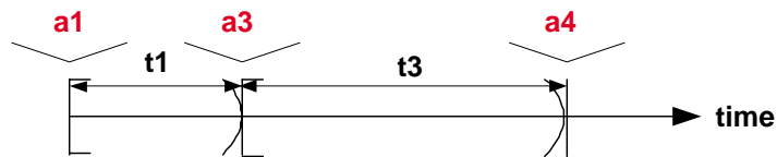
Figure 1.4 A timed trace of the transition system
