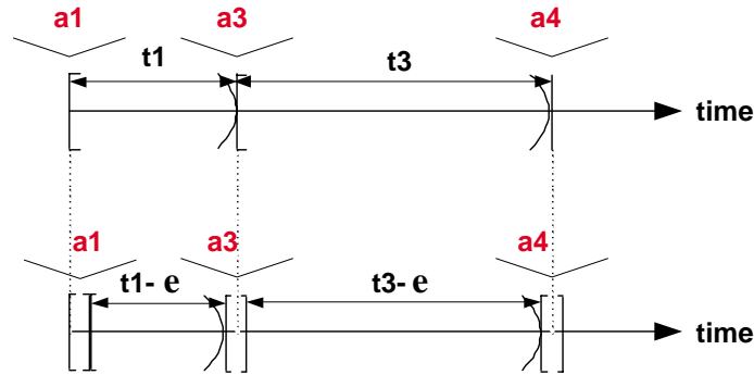
Figure 1.8 Timed traces \epsilon -close
